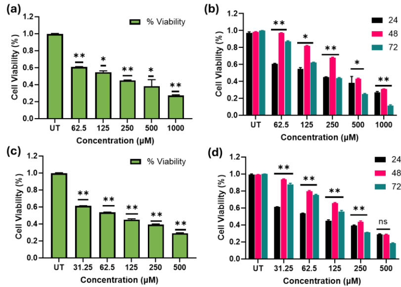
Figure 2: Cytotoxicity of Imatinib and Naringin treated to the K562-S cell lines (a) Imatinib treatment for a period of 24 hours (b) Imatinib treatment for a period of 24 -72 hours (c) Naringin treatment for a period of 24 hours (d) Naringin treatment for a period of 24-72 hours. As the experimentations are made in triplicates (n = 3) statistical analysis representations, * = P < 0.001 ; ** = P < 0.05 ; ns = P > 0.05
