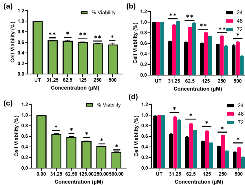
Figure 3: Cytotoxicity of Imatinib and Naringin treated to the K562-R cell lines (a) Imatinib treatment for a period of 24 hours (b) Imatinib treatment for a period of 24 -72 hours (c) Naringin treatment for a period of 24 hours (d) Naringin treatment for a period of 24-72 hours. As the experimentations are made in triplicates (n = 3) statistical analysis representations, * = P < 0.001 ; ** = P < 0.05 ; ns = P > 0.05
